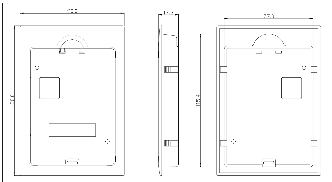
Fig 2-3 Installation box dimension
