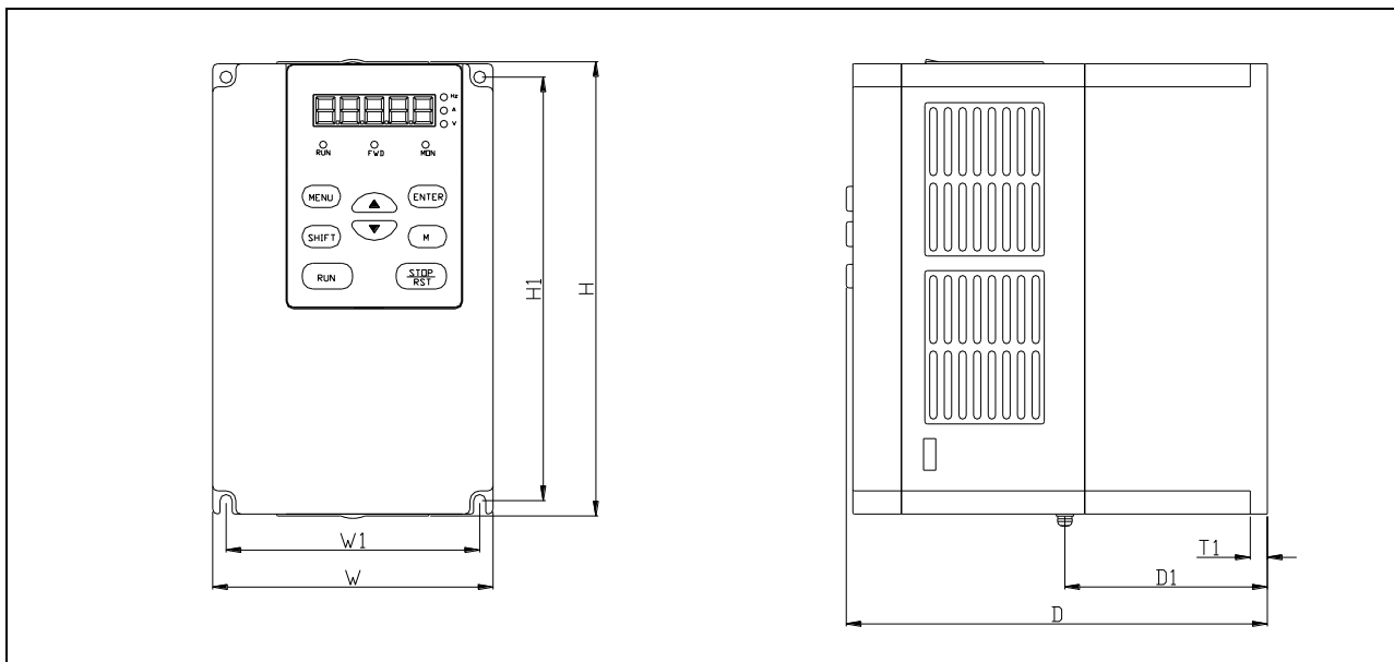
Fig 2-1 FV100-4T-0037G/0055L and lower power VFD
