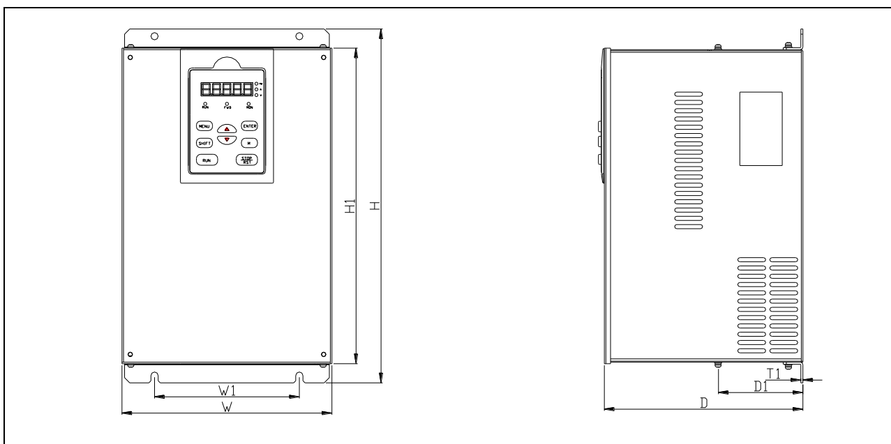
Fig 2-2 FV100-4T-0055G/0075L~FV100-4T-4000G/4500L
