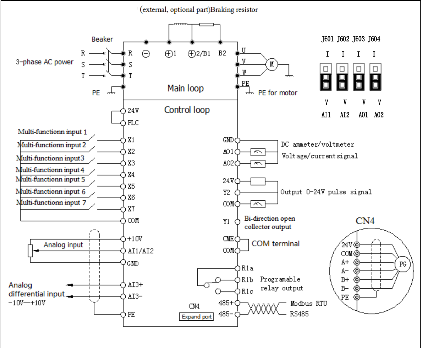
Fig.4-1 Basic wiring chart
