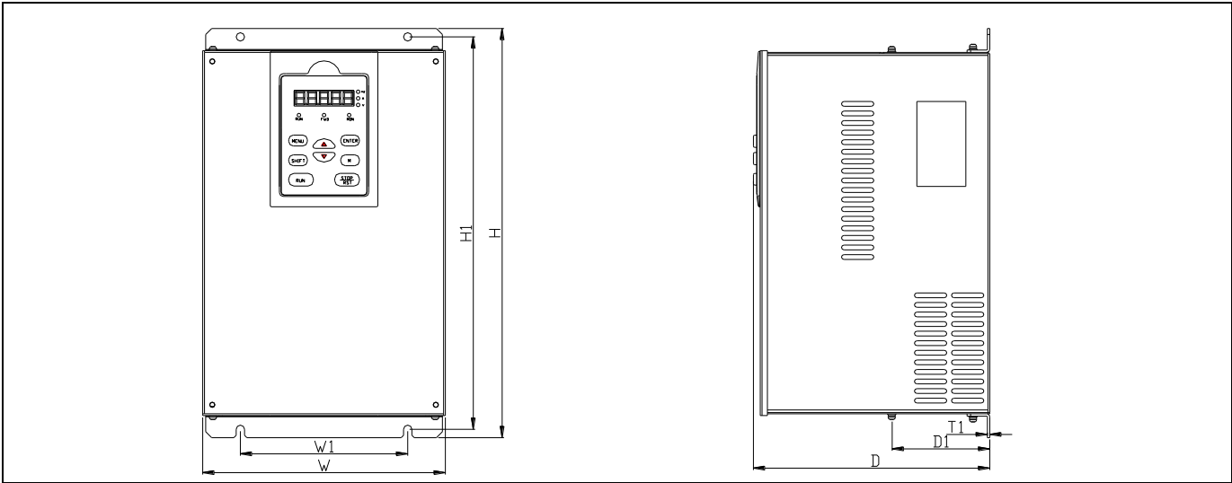
图 2-2 FV100-4T-0055G/0075L~FV100-4T-4000G/4500L
